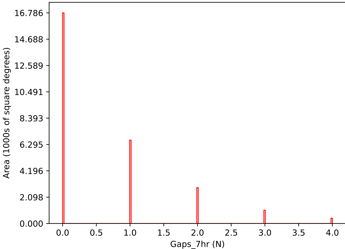
weather_cloudso0v3.4_10yrs i band: Gaps_7hr
