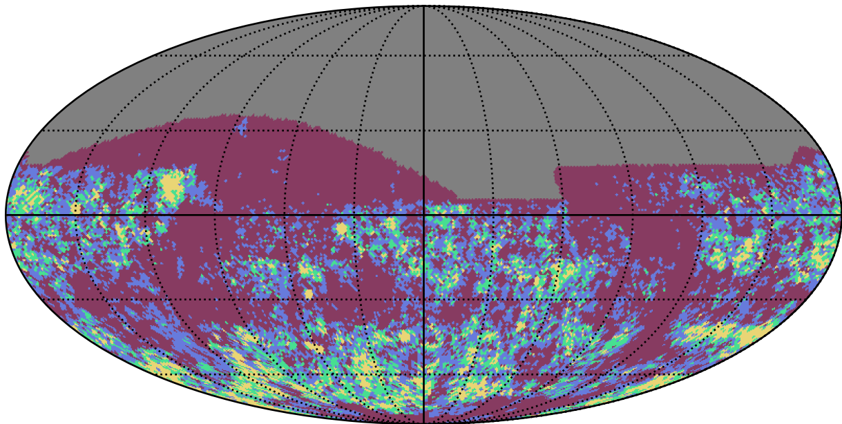
weather_cloudso0v3.4_10yrs z band: Gaps_3hr
