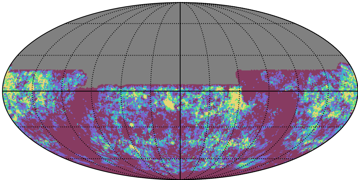
weather_cloudso0v3.4_10yrs y band: Gaps_3hr
