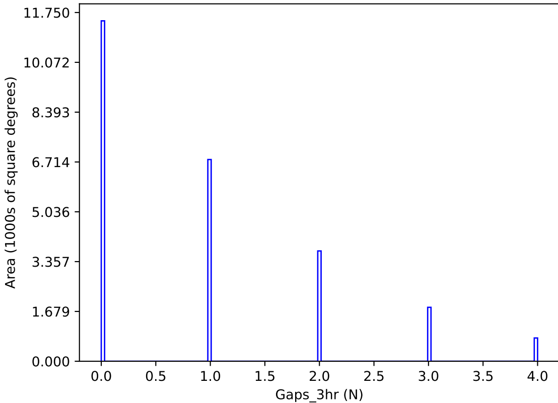
weather_cloudso0v3.4_10yrs y band: Gaps_3hr
