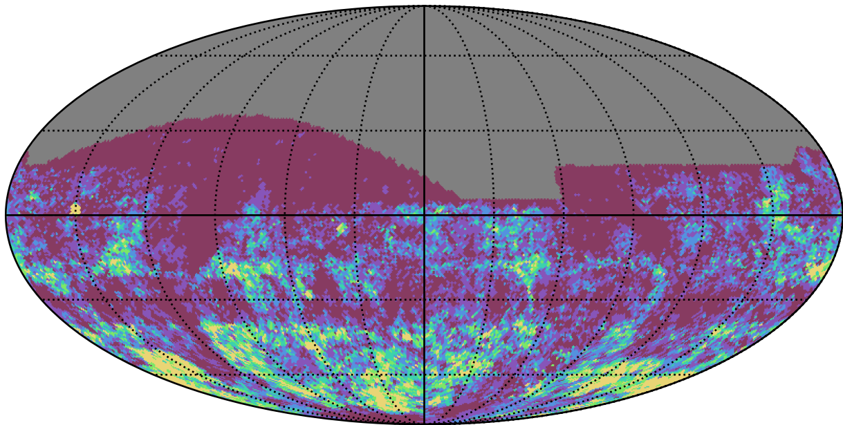
weather_cloudso0v3.4_10yrs r band: Gaps_3hr
