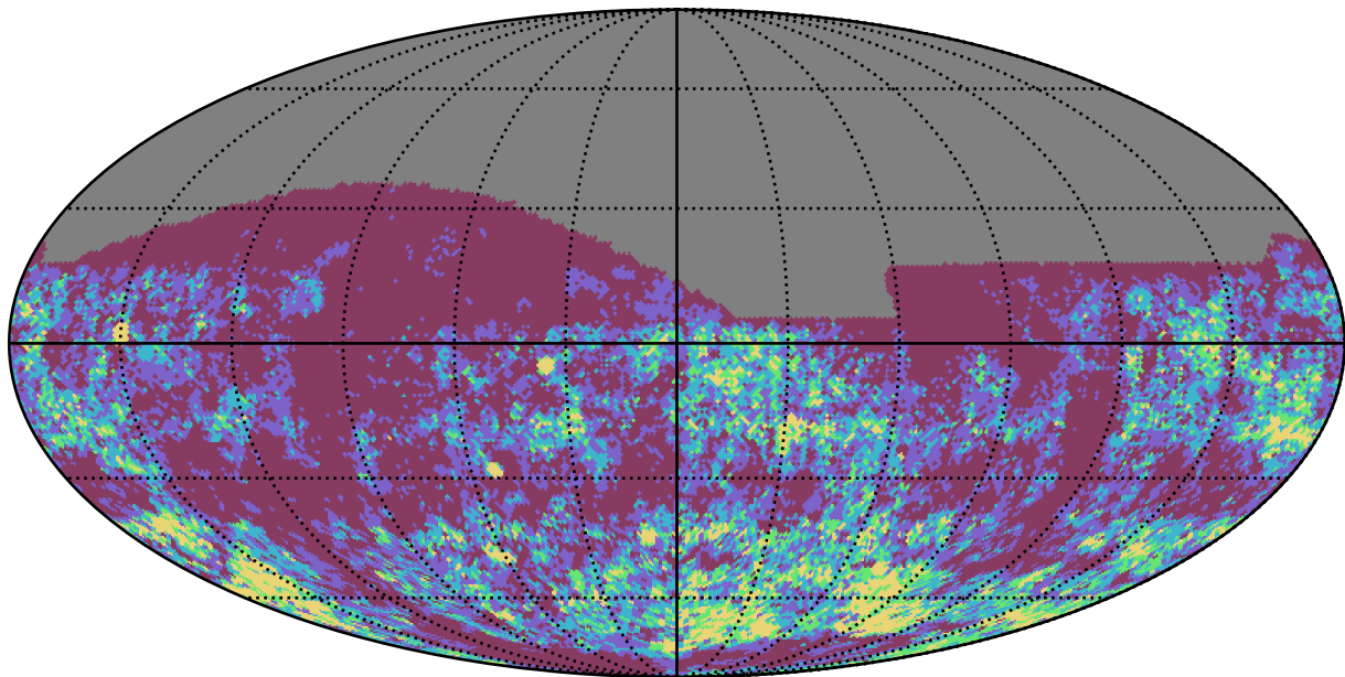
weather_cloudso0v3.4_10yrs i band: Gaps_3hr
