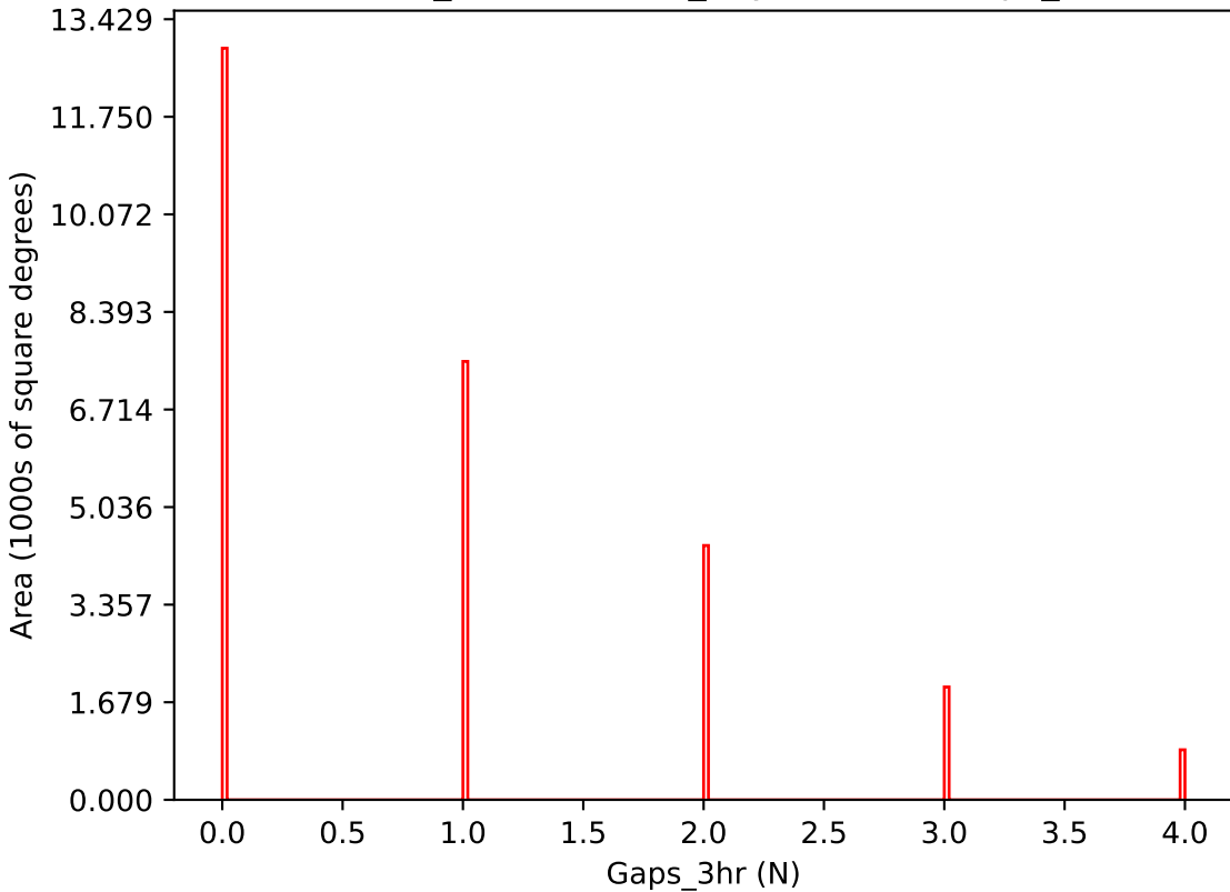
weather_cloudso0v3.4_10yrs i band: Gaps_3hr
