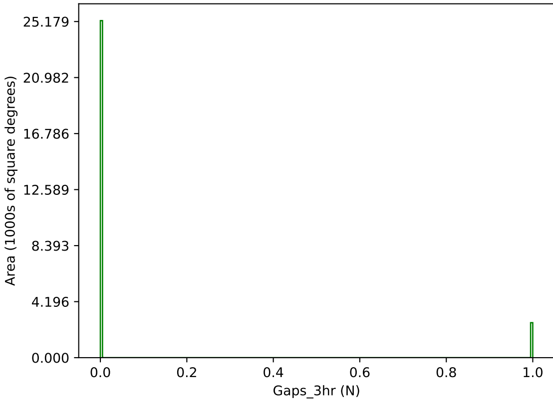
weather_cloudso0v3.4_10yrs g band: Gaps_3hr
