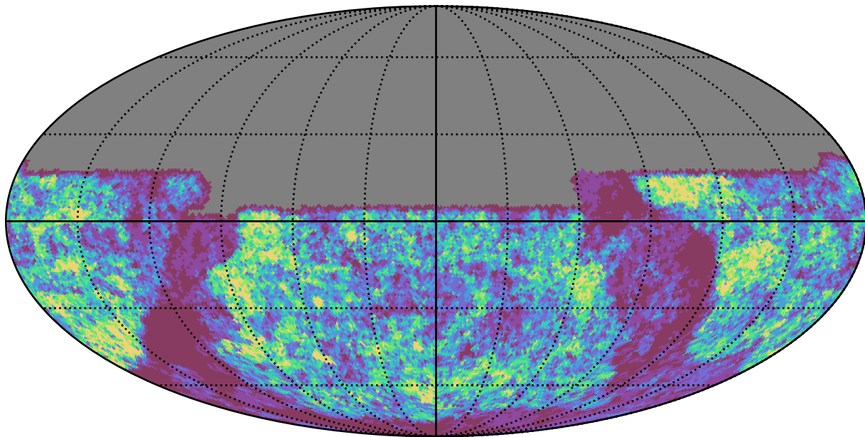
weather_cloudso0v3.4_10yrs u band: Gaps_24hr
