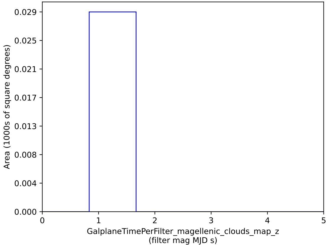
weather_cloudso0v3.4_10yrs : GalplaneTimePerFilter_magellenic_clouds_map_z
