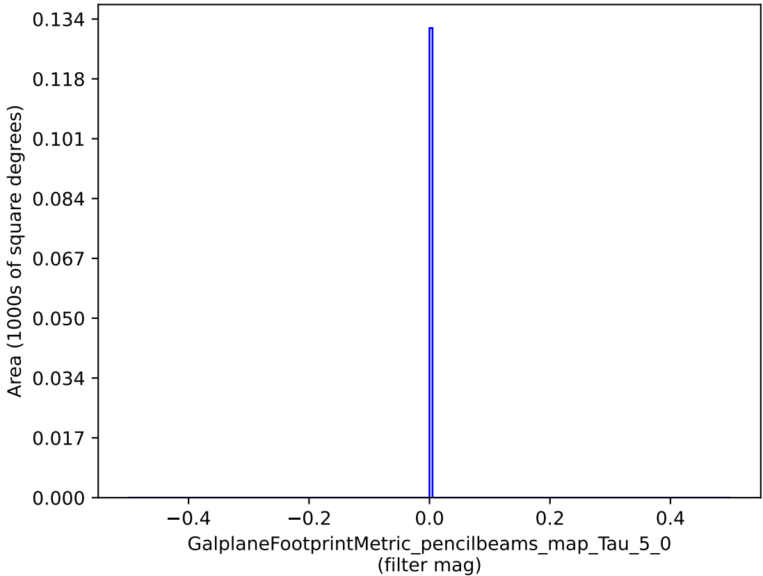
weather_cloudso0v3.4_10yrs : GalplaneFootprintMetric_pencilbeams_map_Tau_5_0
