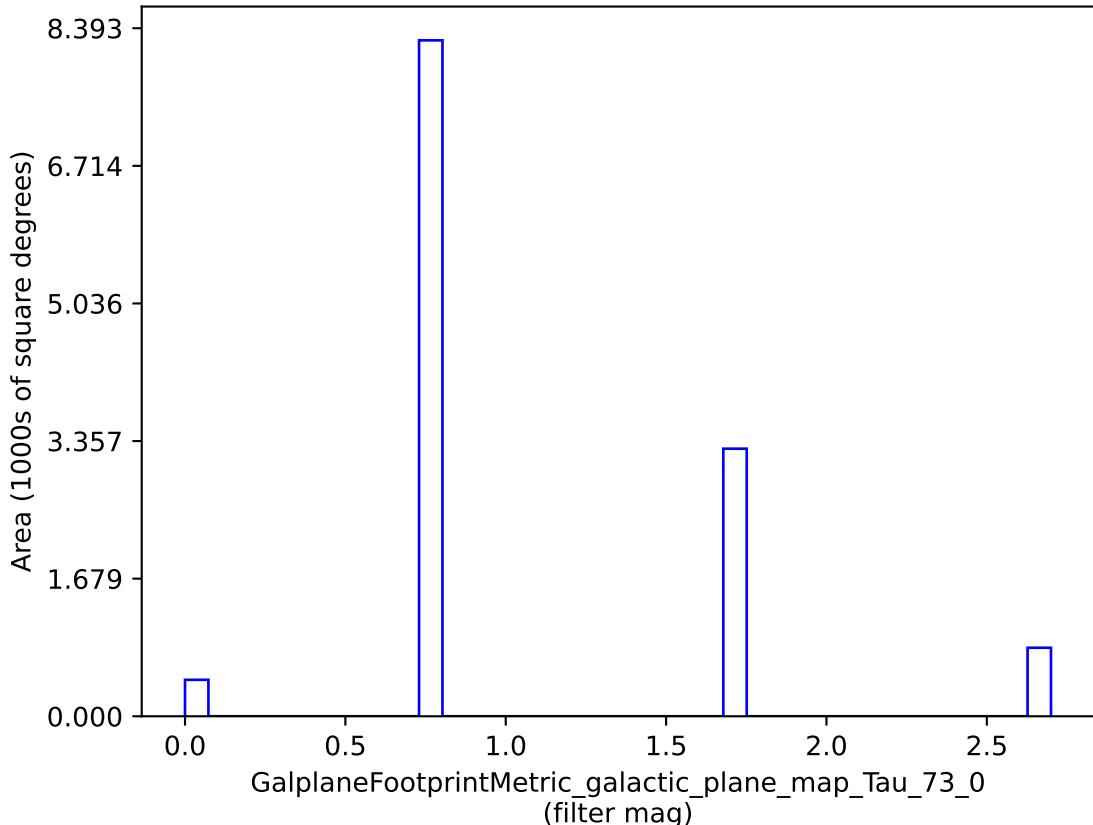
weather_cloudso0v3.4_10yrs : GalplaneFootprintMetric_galactic_plane_map_Tau_73_0
