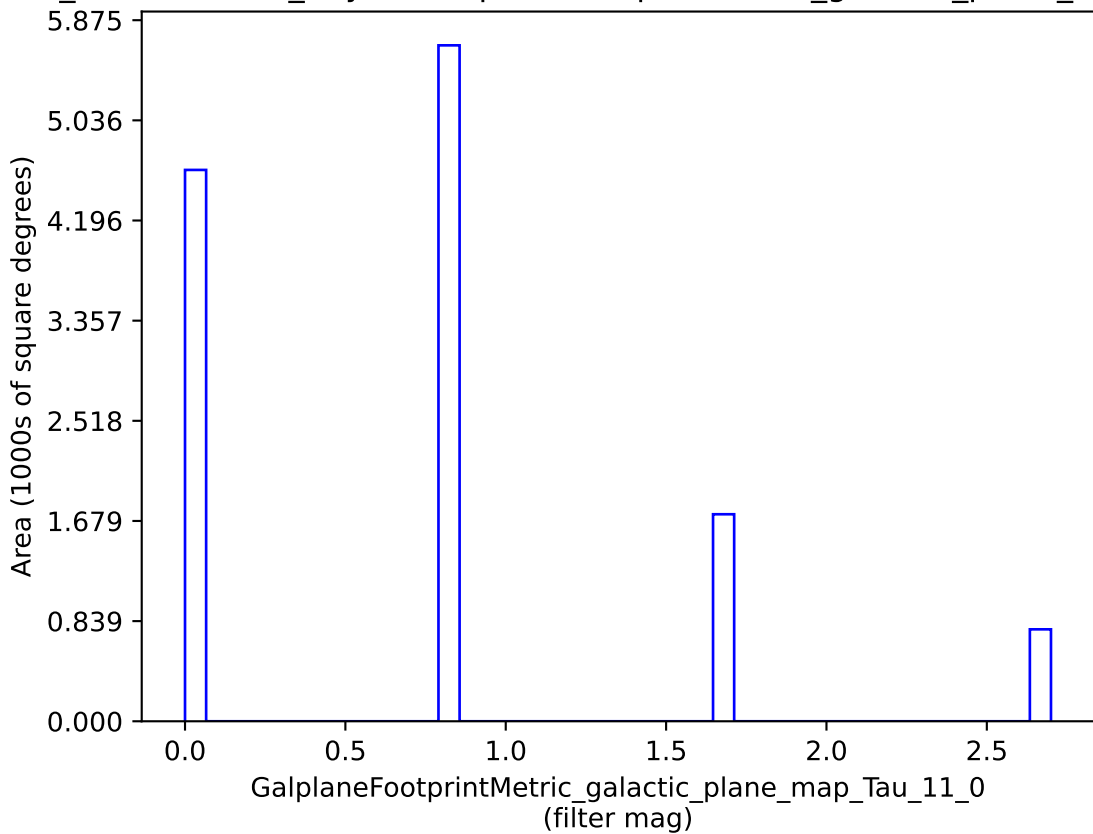
weather_cloudso0v3.4_10yrs : GalplaneFootprintMetric_galactic_plane_map_Tau_11_0
