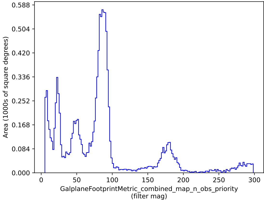
weather_cloudso0v3.4_10yrs : GalplaneFootprintMetric_combined_map_n_obs_priority
