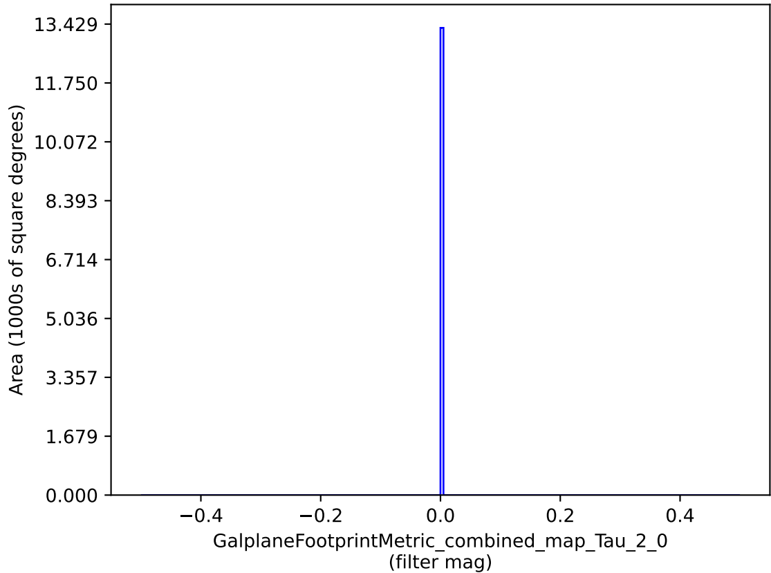
weather_cloudso0v3.4_10yrs : GalplaneFootprintMetric_combined_map_Tau_2_0
