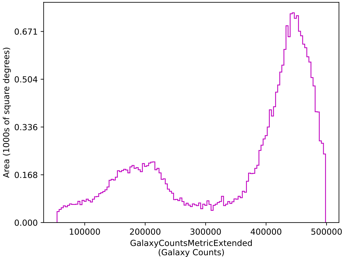
weather_cloudso0v3.4_10yrs z: GalaxyCountsMetricExtended
