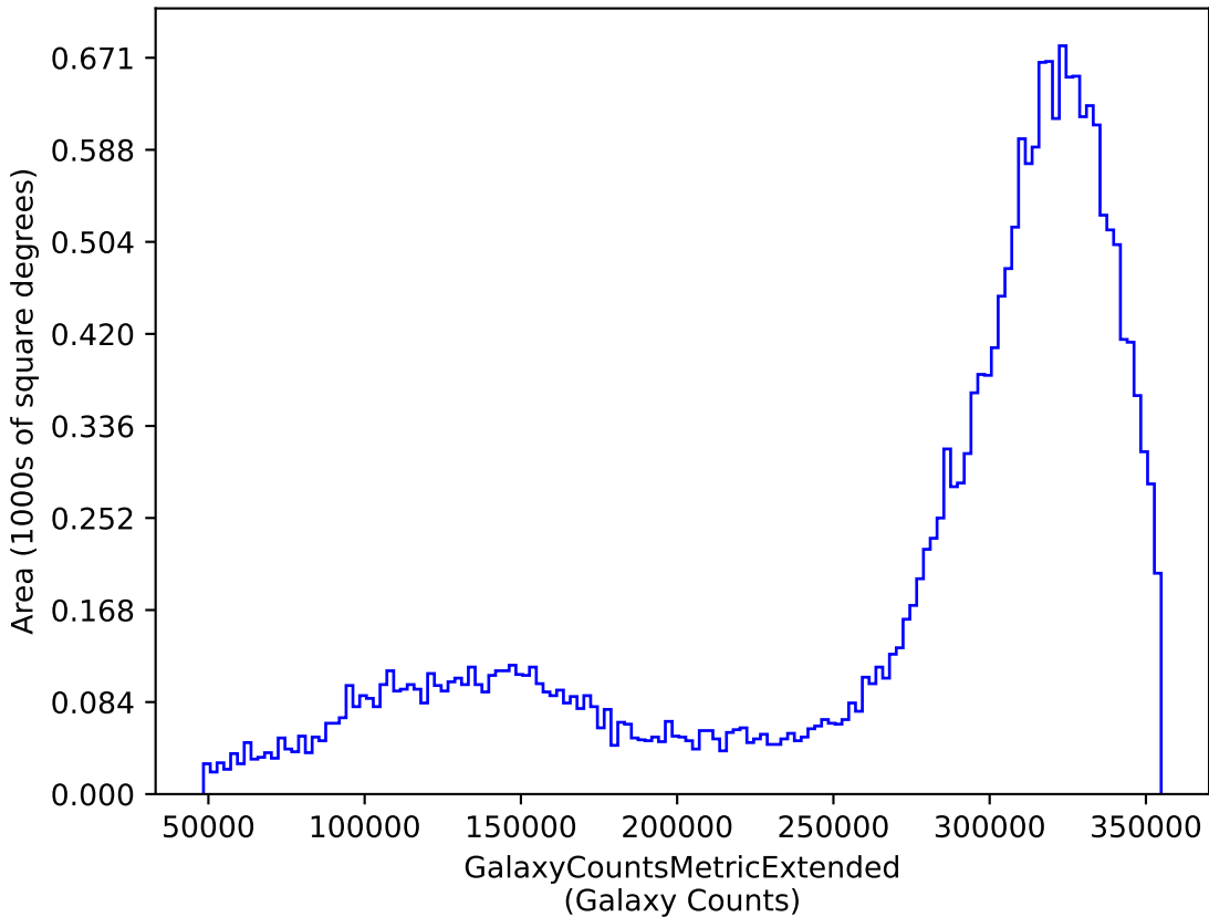
weather_cloudso0v3.4_10yrs y: GalaxyCountsMetricExtended
