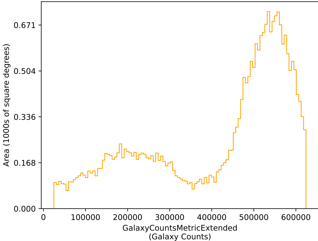
weather_cloudso0v3.4_10yrs r: GalaxyCountsMetricExtended
