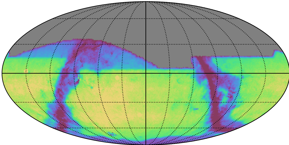
weather_cloudso0v3.4_10yrs i: GalaxyCountsMetricExtended
