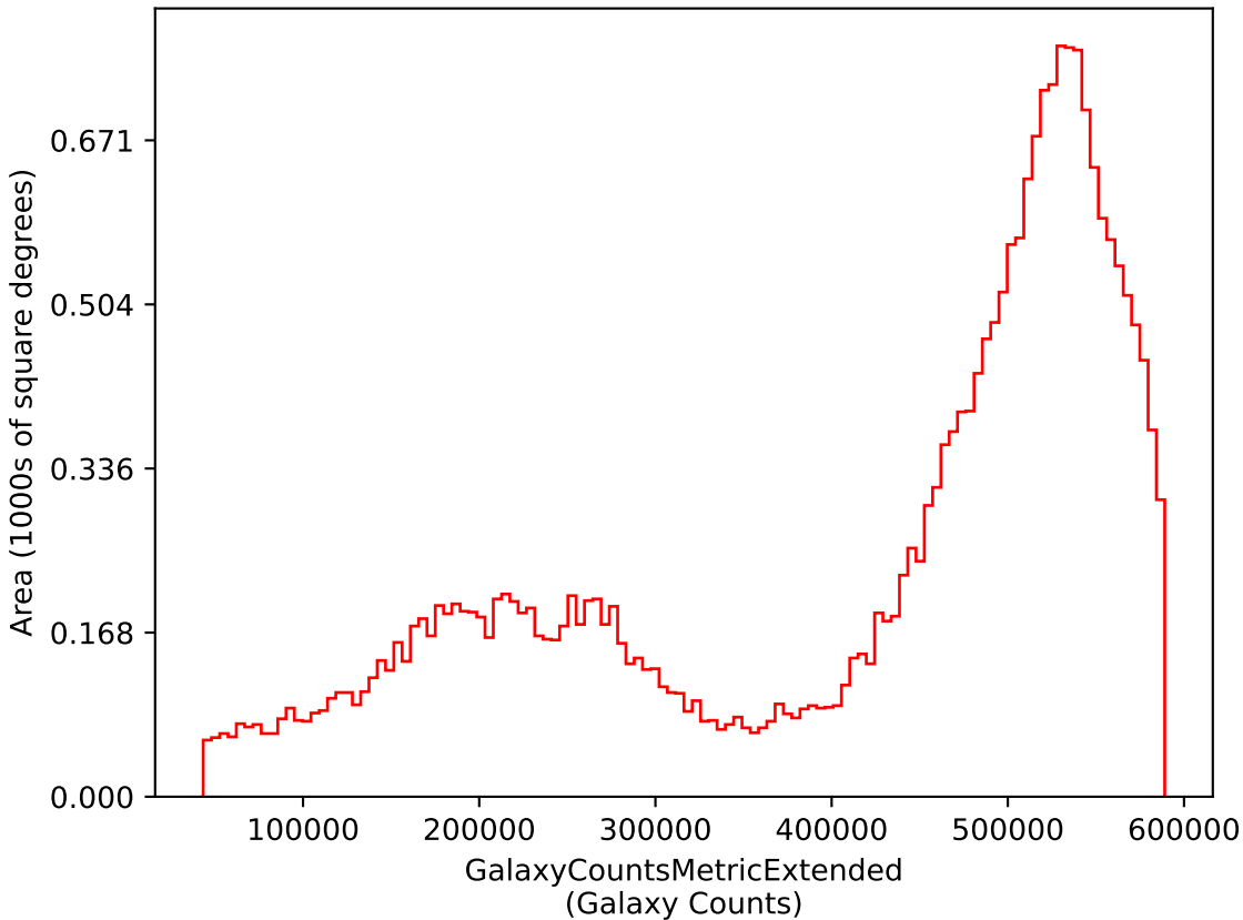
weather_cloudso0v3.4_10yrs i: GalaxyCountsMetricExtended
