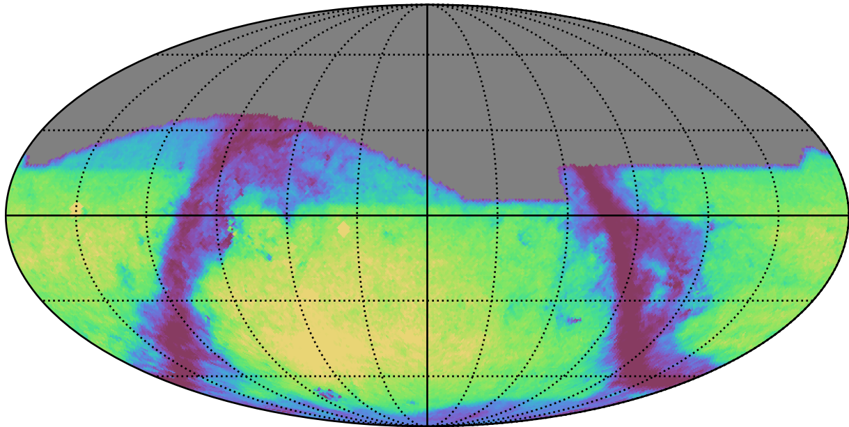
weather_cloudso0v3.4_10yrs g: GalaxyCountsMetricExtended
