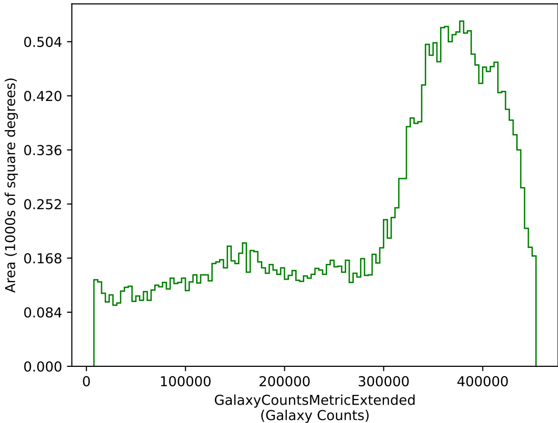
weather_cloudso0v3.4_10yrs g: GalaxyCountsMetricExtended
