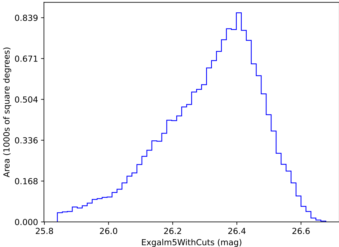
weather_cloudso0v3.4_10yrs i band non-DD year 9: Exgalml5WithCuts
