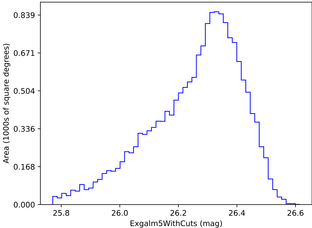
weather_cloudso0v3.4_10yrs i band non-DD year 8: Exgalml5WithCuts
