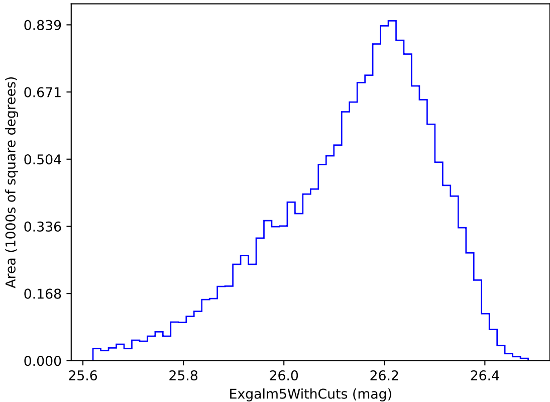
weather_cloudso0v3.4_10yrs i band non-DD year 6: Exgalml5WithCuts
