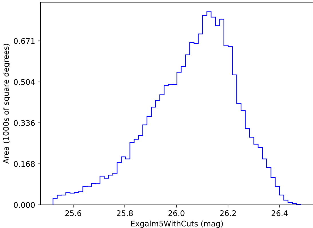
weather_cloudso0v3.4_10yrs i band non-DD year 5: Exgalml5WithCuts
