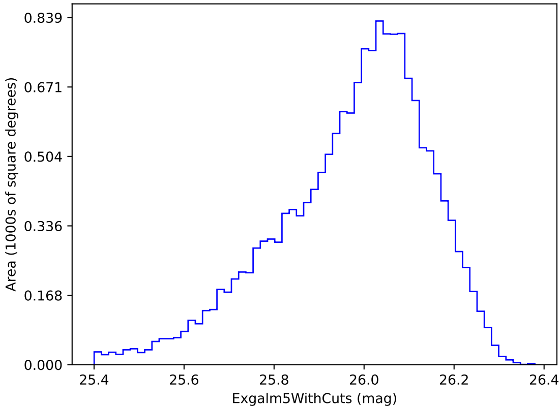
weather_cloudso0v3.4_10yrs i band non-DD year 4: Exgalml5WithCuts
