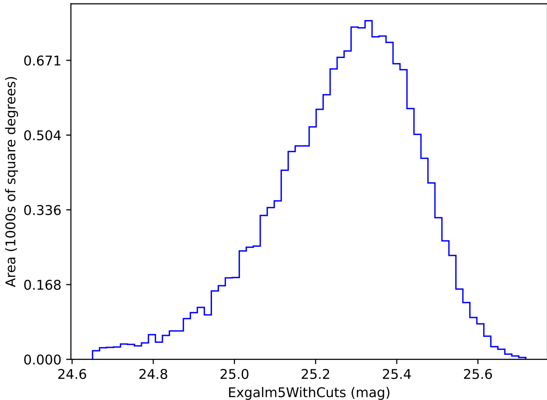
weather_cloudso0v3.4_10yrs i band non-DD year 1: Exgalml5WithCuts
