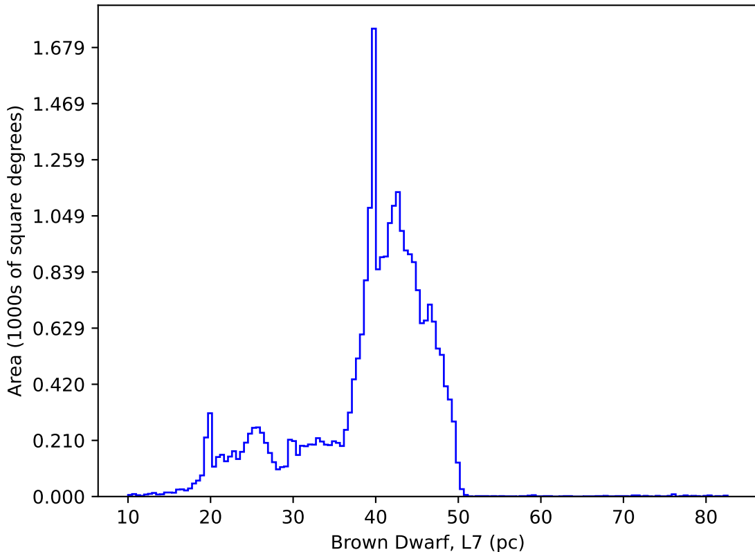
weather_cloudso0v3.4_10yrs : Brown Dwarf, L7
