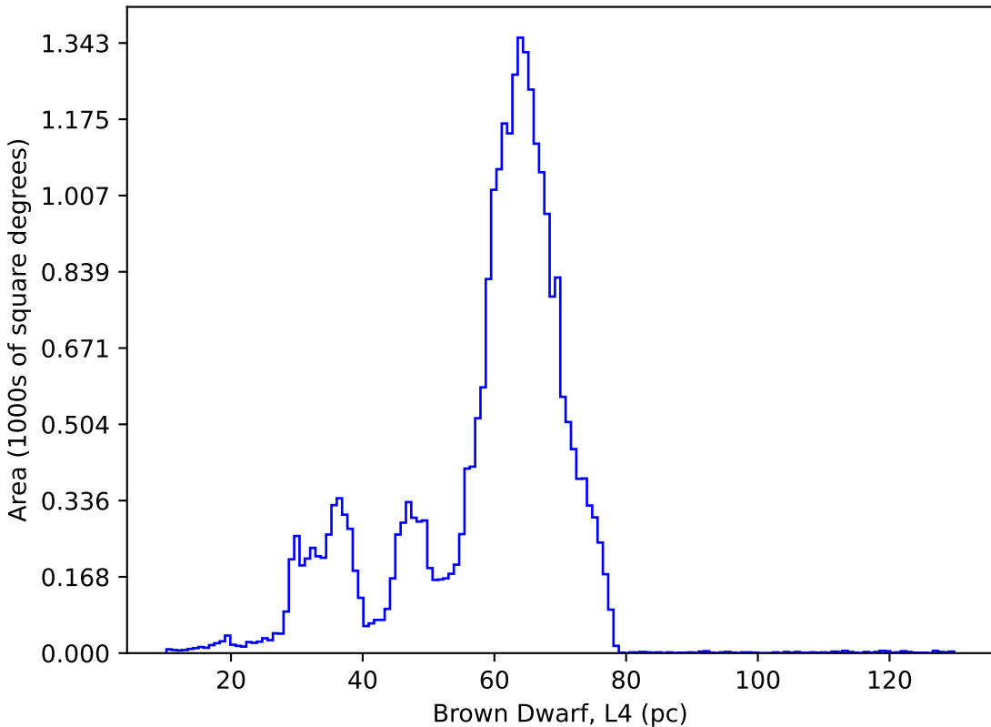
weather_cloudso0v3.4_10yrs : Brown Dwarf, L4
