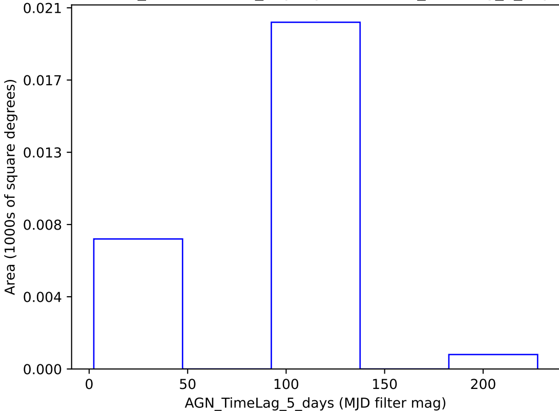
weather_cloudso0v3.4_10yrs y band: AGN_TimeLag_5_days
