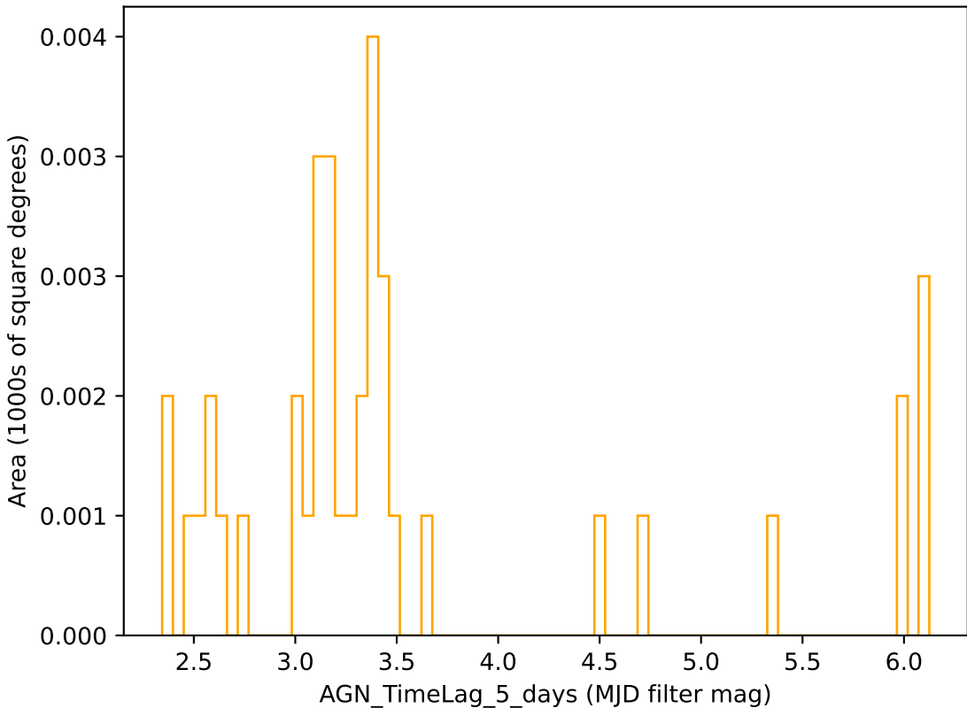
weather_cloudso0v3.4_10yrs r band: AGN_TimeLag_5_days
