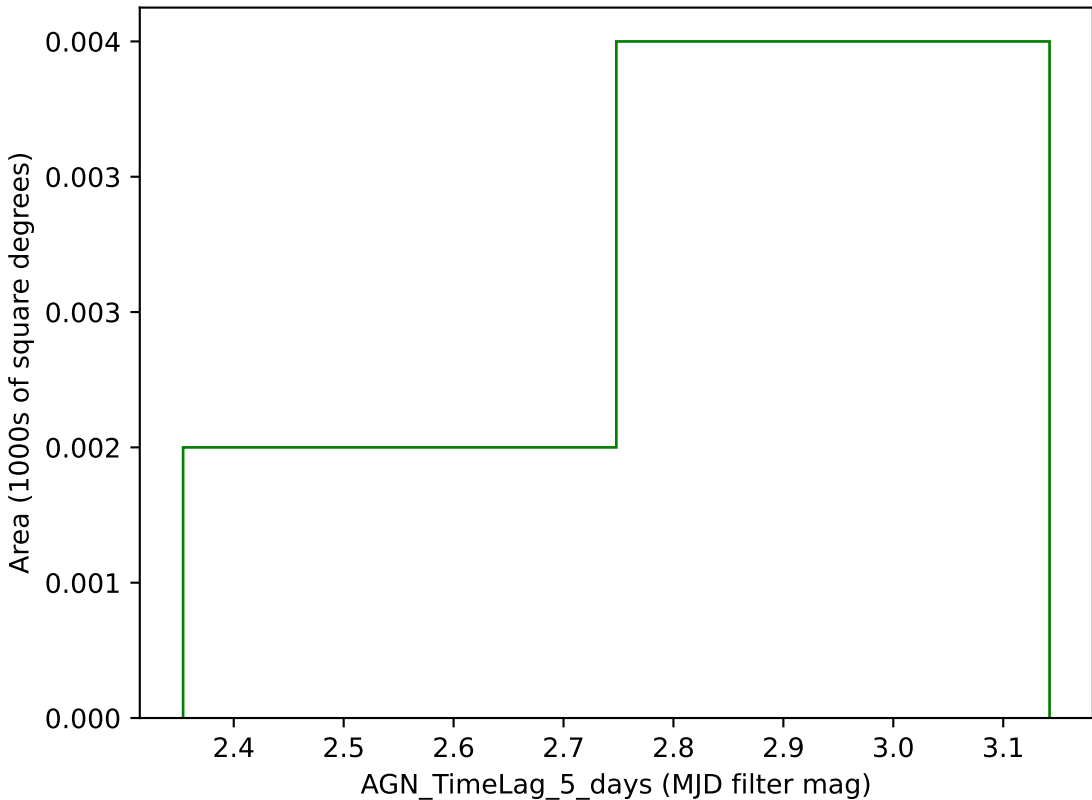
weather_cloudso0v3.4_10yrs g band: AGN_TimeLag_5_days
