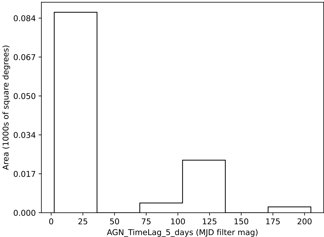
weather_cloudso0v3.4_10yrs all bands: AGN_TimeLag_5_days
