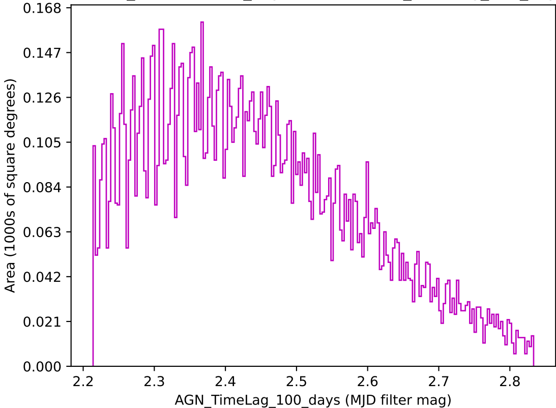
weather_cloudso0v3.4_10yrs z band: AGN_TimeLag_100_days
