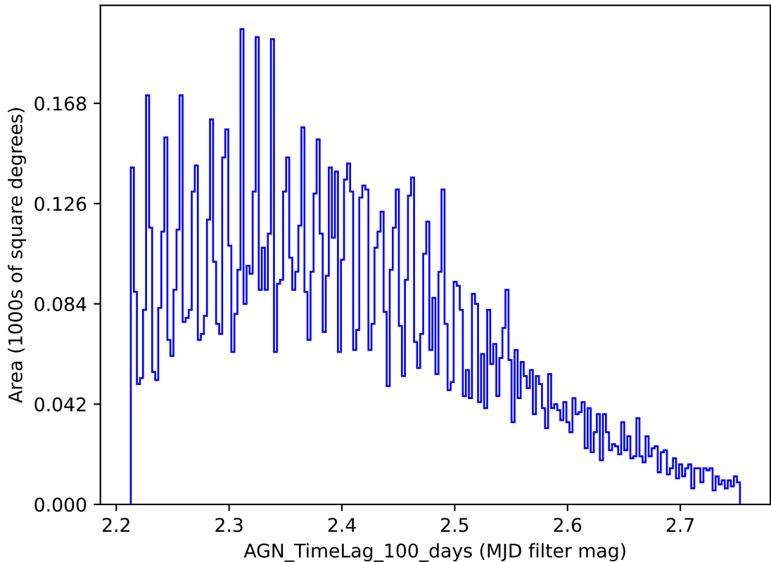
weather_cloudso0v3.4_10yrs y band: AGN_TimeLag_100_days
