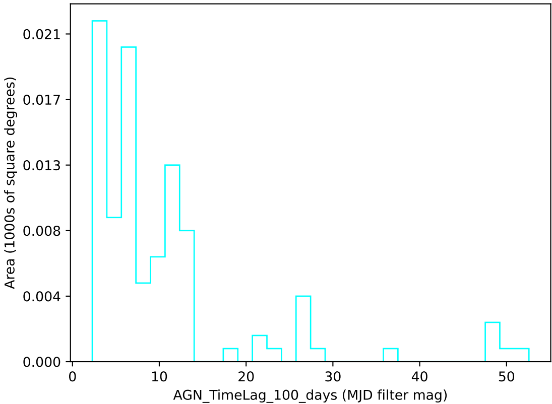
weather_cloudso0v3.4_10yrs u band: AGN_TimeLag_100_days
