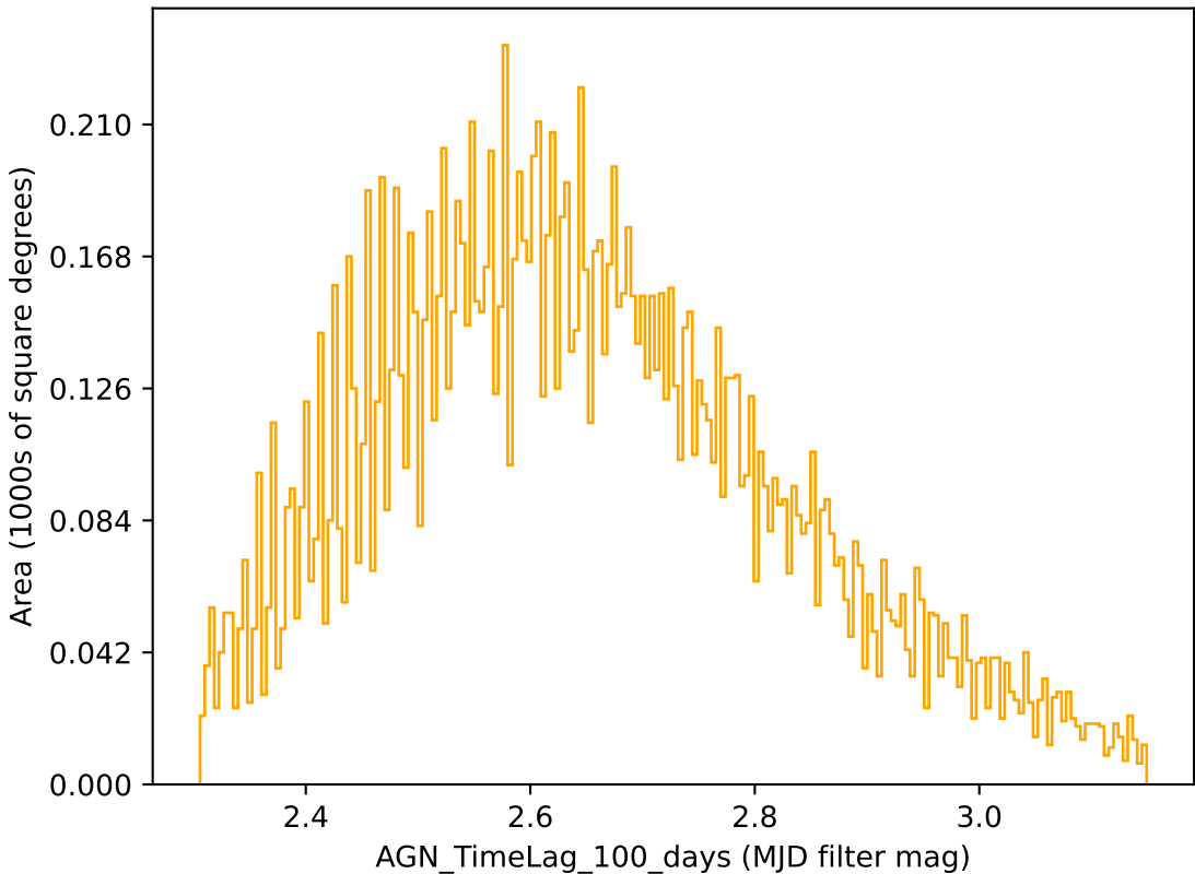
weather_cloudso0v3.4_10yrs r band: AGN_TimeLag_100_days
