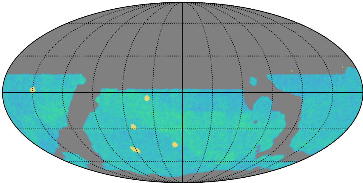
weather_cloudso0v3.4_10yrs i band: AGN_TimeLag_100_days
