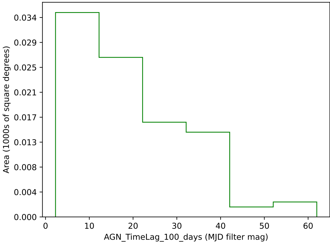
weather_cloudso0v3.4_10yrs g band: AGN_TimeLag_100_days
