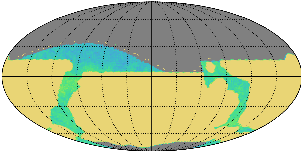
weather_cloudso0v3.4_10yrs all bands: AGN_TimeLag_100_days
