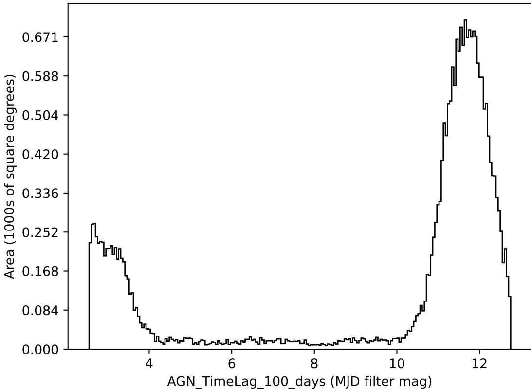
weather_cloudso0v3.4_10yrs all bands: AGN_TimeLag_100_days
