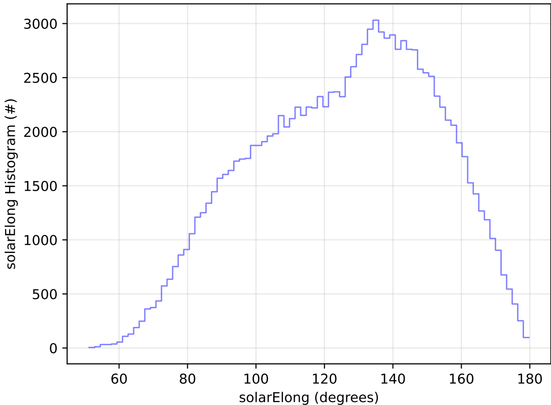
weather_cloudso0v3.4_10yrs WFD u band: solarElong Histogram
