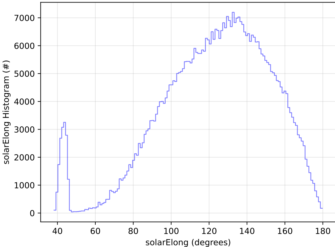
weather_cloudso0v3.4_10yrs WFD r band: solarElong Histogram
