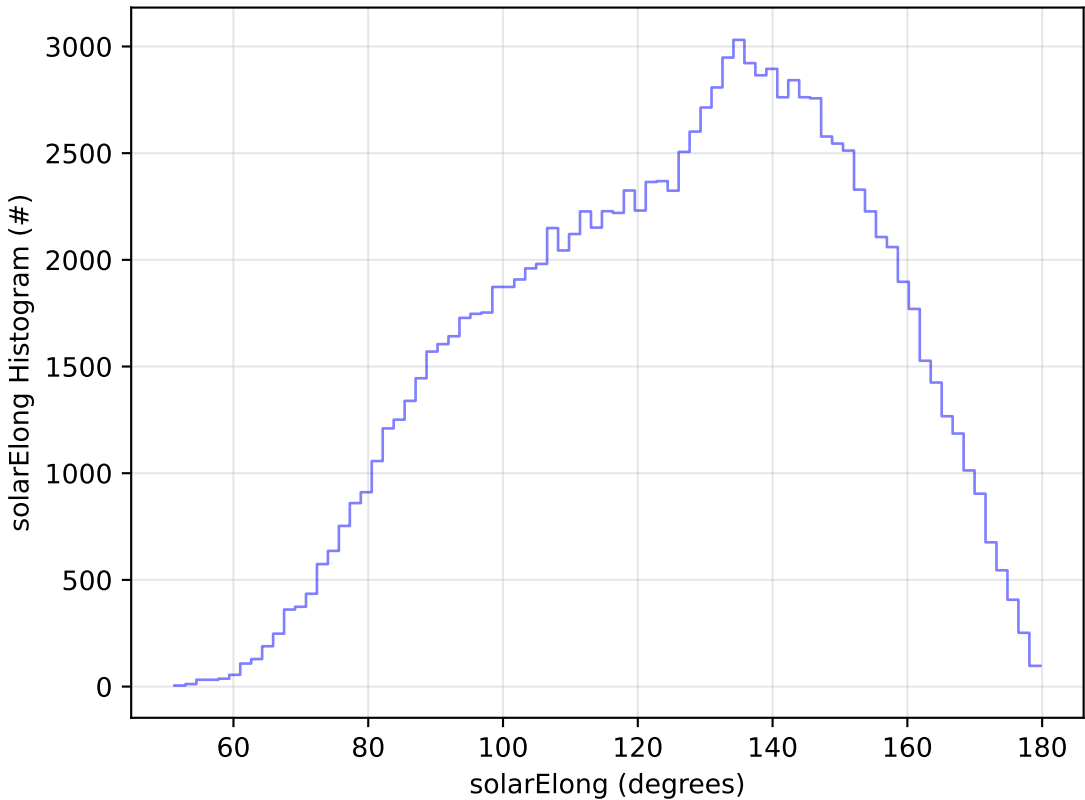
weather_cloudso0v3.4_10yrs All sky u band: solarElong Histogram
