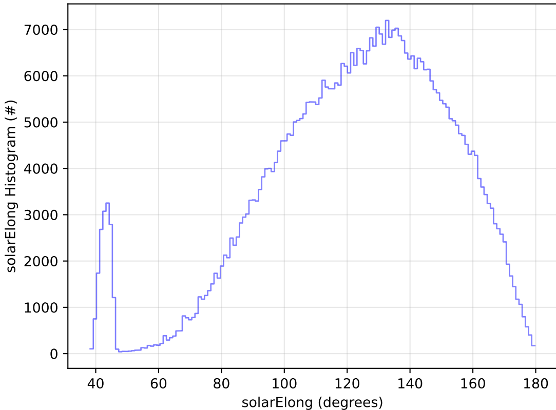
weather_cloudso0v3.4_10yrs All sky r band: solarElong Histogram
