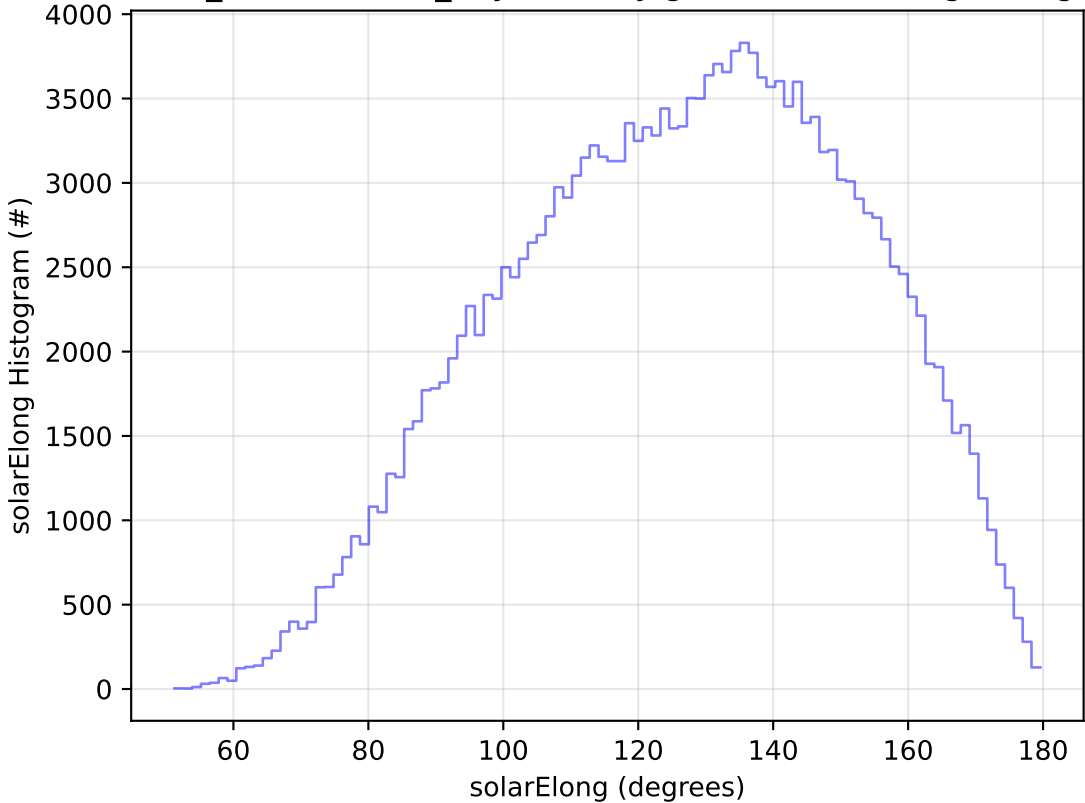
weather_cloudso0v3.4_10yrs All sky g band: solarElong Histogram
