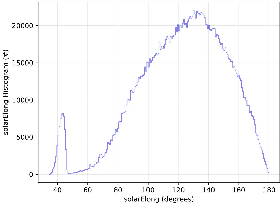
weather_cloudso0v3.4_10yrs All sky all bands: solarElong Histogram
