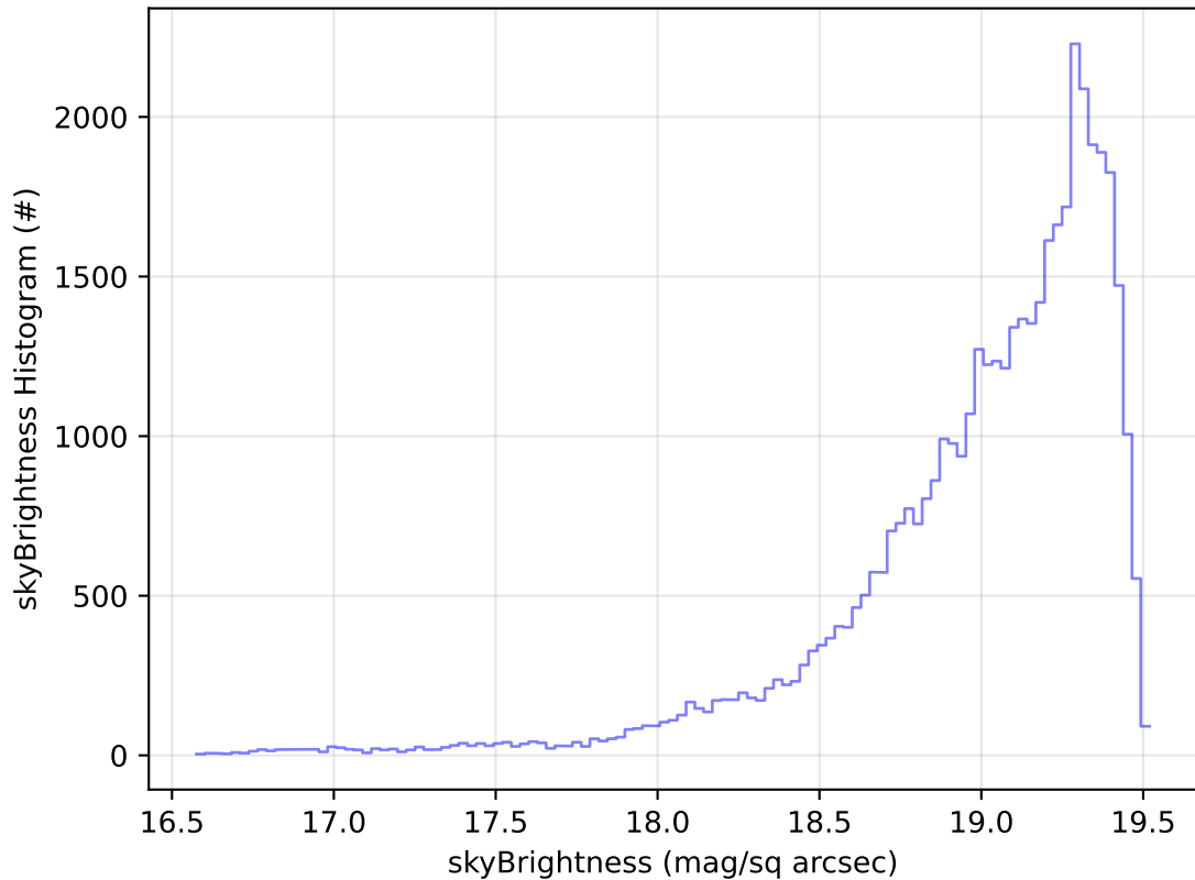
weather_cloudso0v3.4_10yrs Yr 1 z band: skyBrightness Histogram
