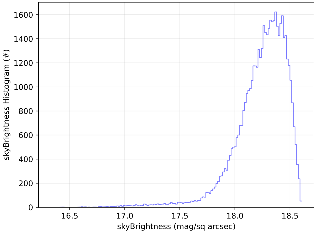
weather_cloudso0v3.4_10yrs Yr 1 y band: skyBrightness Histogram
